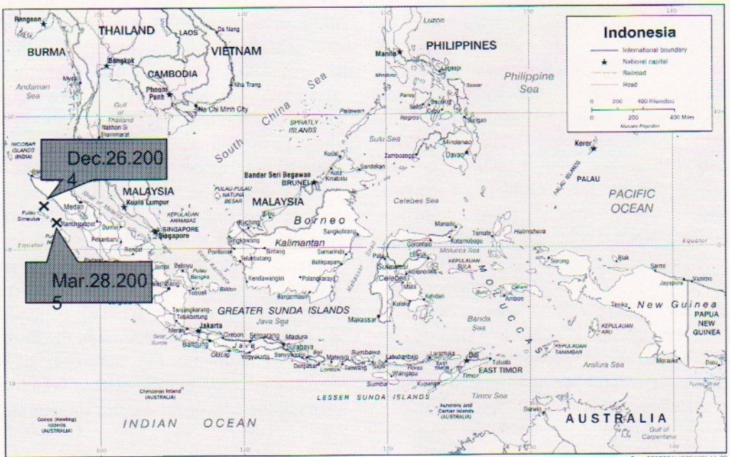
Fig. 1. Locations of the large tsunami occurrence around Aceh, Indonesia in 2004 and 2005
