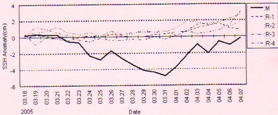
Fig. 6. As in Fig. 5, but for the tsunami occurred on March 28 th , 2005
