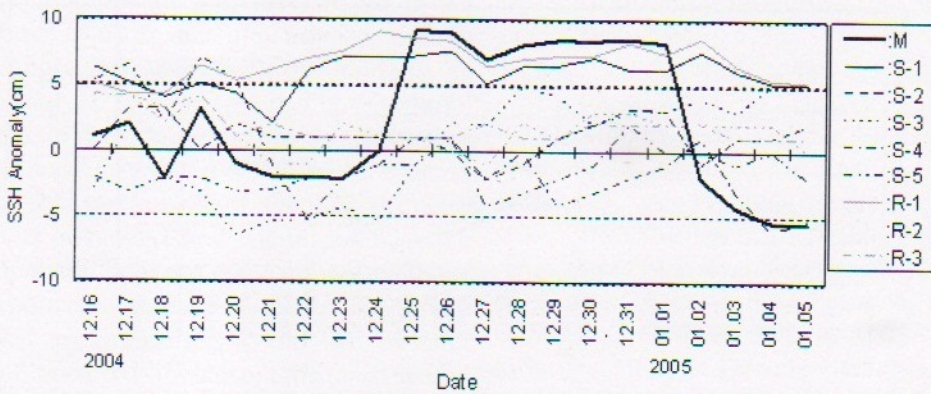
Fig. 5. Time series of sea surface height anomaly from December 16 th , 2004 to January 5 th , 2005 for tsunami event on December 26 th , 2004. Each line can be referred to the time scale for the grid as shown in the legend.
