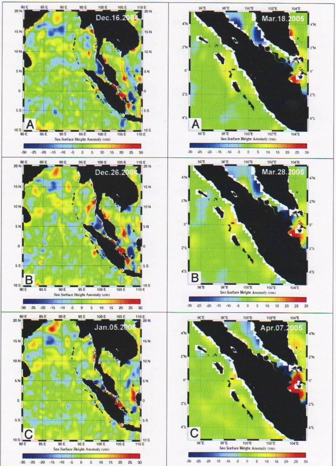
Fig. 3. Images of sea surface height anomaly obtained the date before(A), just(B), and after(C) the tsunami event. Left and right figures are corresponding to the event occurred on December 26 th 2004 and March 28 th 2005, respectively
