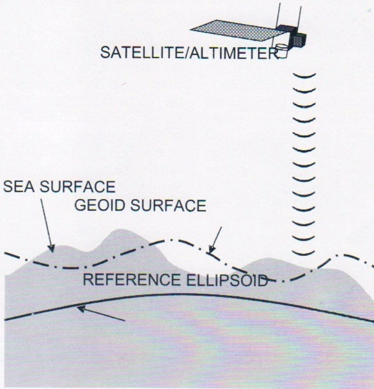
Fig. 2. Schematic representation of the concept for sea surface height measurement by satellite-borne altimeter
