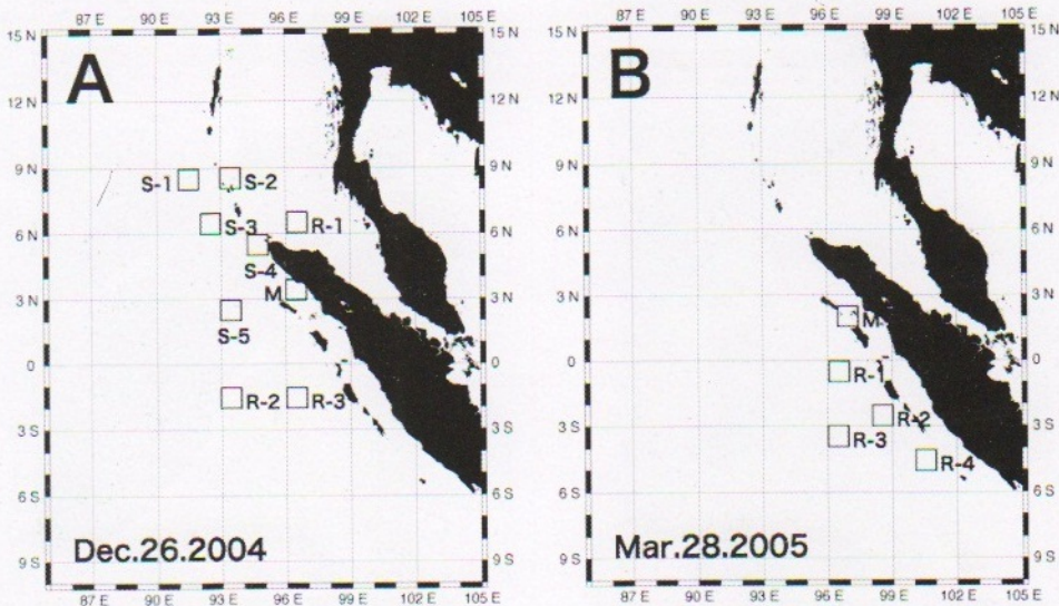
Fig. 4. Grids set for the trace of change in sea surface height anomaly from ten days before to ten days after the tsunami events occurred on December 26 th , 2004 (A) and March 28 th , 2005 (B). Initial letters of the grid index, "M", "S", and "R" are defined as the grid including hypocenter, aftershock, and no earthquake, respectively
