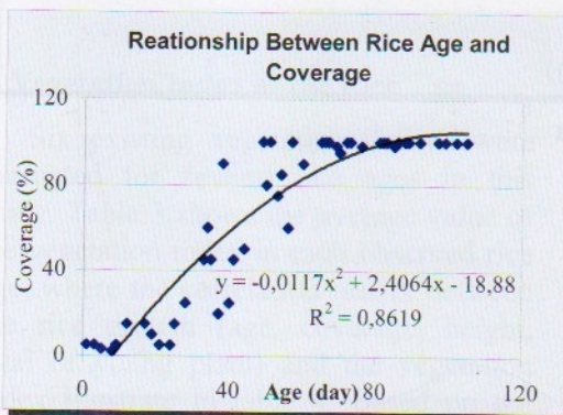
Fig. 2. Relationship between rice growth parameters and age of the rice
