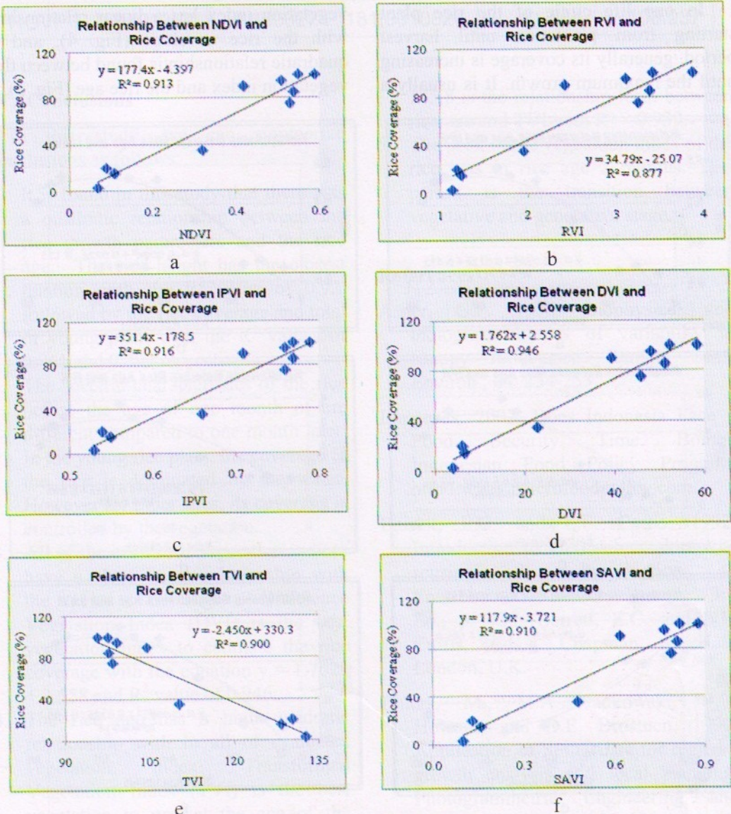
Fig. 4. Linear relationship between vegetation index and rice coverage
