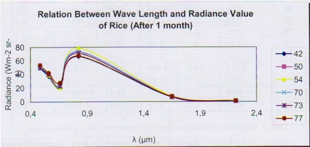
Fig. 3. Relationship between radian value and wave length in several rice age
